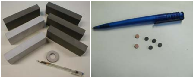
Fig. 8. Magnet sensors and UHF ferrites coated by low pressure cold spray process.
