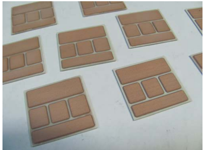
Fig. 7. Contact pads at AlN ceramic plates deposited by gas dynamic spray.
